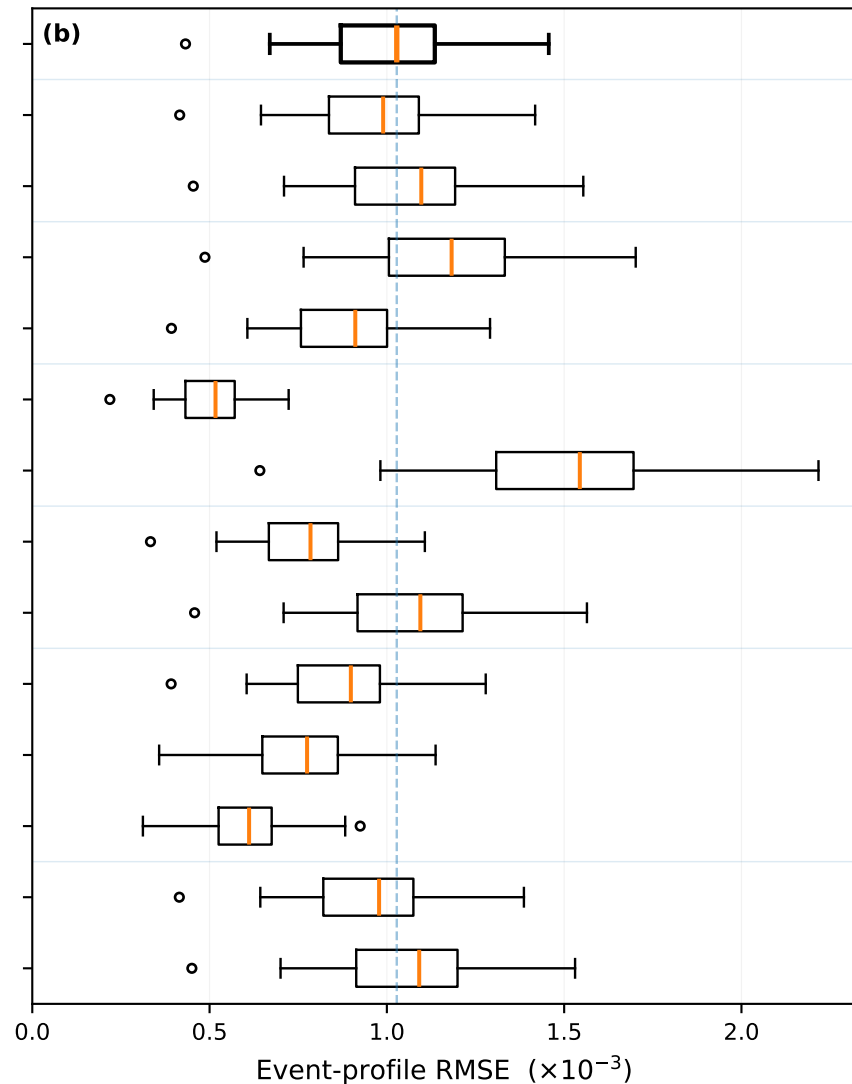
Non-parametric recovery
