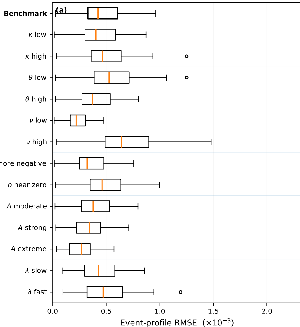
Parametric recovery
